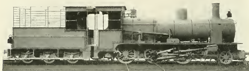
GERMAN MOGUL FOR ASSAM RAILWAY, BENGAL.
